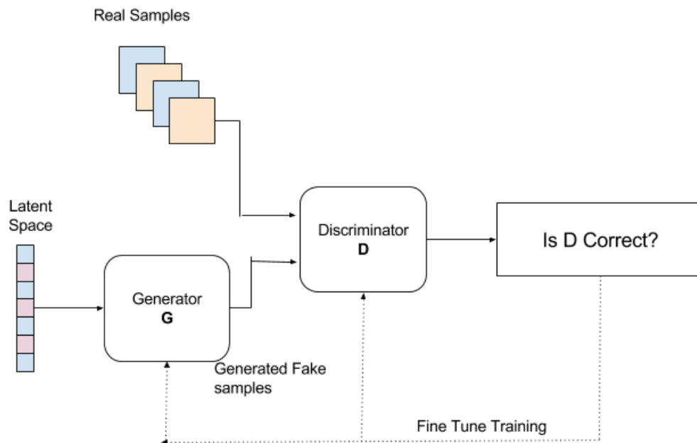
Fig. 3.6. Architecture of a Generative Adversarial Network. The generator G takes as input latent variables that he later pass to the discriminator D. The discriminator takes as input the real samples along with the output of the generator and attempts to discriminator between instances that come from the generator and real samples. If D is not correct, G tries to produce data closer to the real data in order to fool D.
